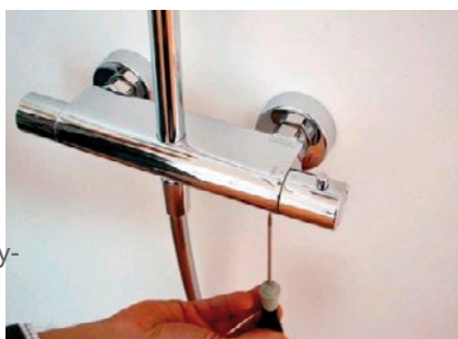
1. Unscrew the grains on the temperature control handle
