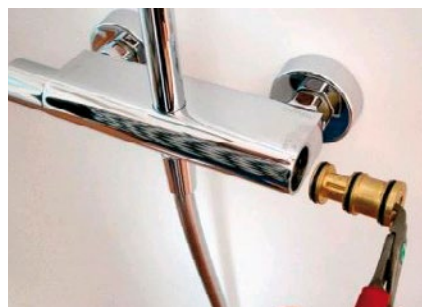
3. Insert the adapter
