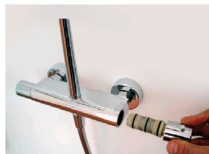
2. Remove existing cartridge and temperature control handle
